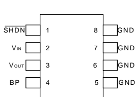
SOP-8 (Top View)
