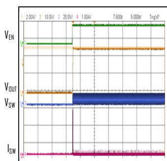
Start-up Waveform with EN VIN=12V, VOUT=5V, IOUT=0A
