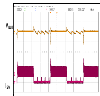
Load Transient Response VIN=12V, VOUT=3.3V, IOUT=0 to 0.5A
