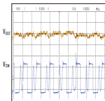
Switching Waveform VIN=12V, VOUT=5V, IOUT=0.1A
