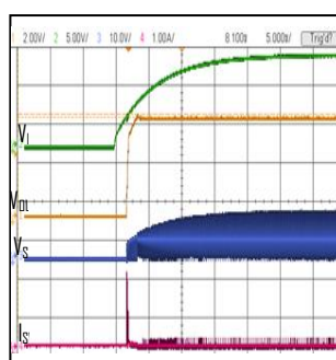
Start-up Waveform with EN=VIN VIN=12V, VOUT=5V, IOUT=0A
