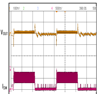
Load Transient Response VIN=12V, VOUT=5V, IOUT=0 to 0.5A
