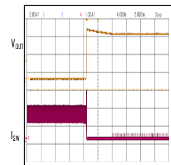
Short-Circuit Recovery VIN=24V, VOUT=5V, IOUT= Short to 0A
