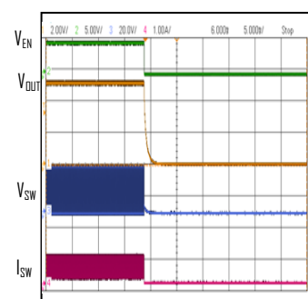
Shutdown Waveform with EN VIN=30V, VOUT=5V, IOUT=0.5A
