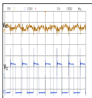
Switching Waveform VIN=12V, VOUT=5V, IOUT=0.3A
