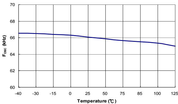
Figure 12. Frequency in Normal Mode (f osc ) vs. Temperature
