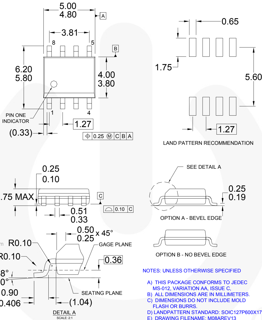
Figure 19. 8-Pin Small Outline Package (SOP)
