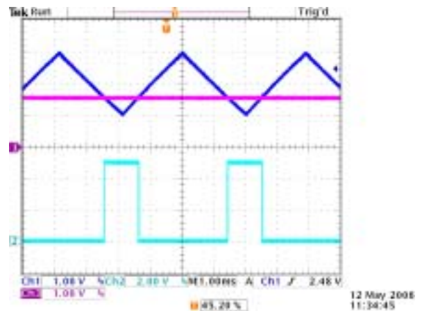
FP5132B Dimming Voltage and PWM Output Waveform
