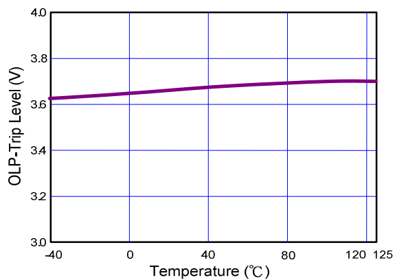
Fig. 5 OLP Trip Level vs. Temperature
