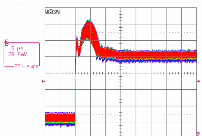
FIGURE 43. LOAD TRANSIENT RESPONSE WITH OVERSHOOT REDUCTION FUNCTION DISABLED, V_{IN} = 12V , SV CLARKSFIELD CPU TEST CONDITION: V_{ID} = 0.95V , I_O = 12A/51A , di/dt = \text{“FASTEST”} , LL = 1.9m\Omega
