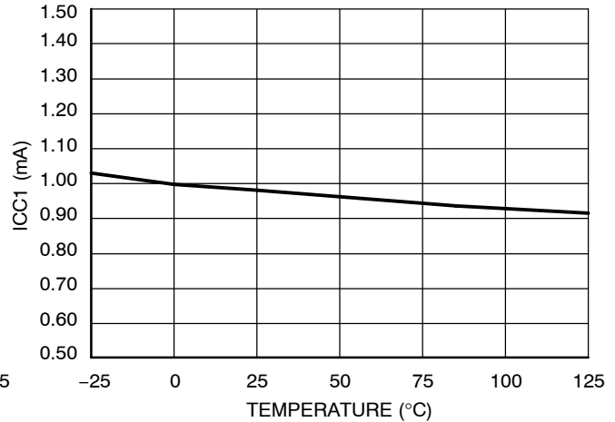
Figure 4. ICC1 @ V_{CC} = 8.0\text{ V} , FB = 1.5 V vs. Temperature
