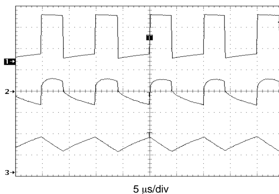
V_{OUT} = 1.9 \text{ V} , V_{in} = 1.2 \text{ V} , I_O = 70 \text{ mA} , L = 47 \text{ } \mu\text{H} , C_{OUT} = 68 \text{ } \mu\text{F} 1. V_{LX} , 1.0 V/div 2. V_{OUT} , 20 mV/div, AC coupled 3. I_L , 100 mA/div
