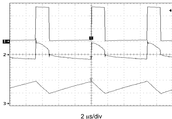
V_{OUT} = 5.0 \text{ V} , V_{in} = 1.5 \text{ V} , I_O = 30 \text{ mA} , L = 47 \text{ } \mu\text{H} , C_{OUT} = 68 \text{ } \mu\text{F} 1. V_{LX} , 2.0 V/div 2. V_{OUT} , 20 mV/div, AC coupled 3. I_L , 100 mA/div
