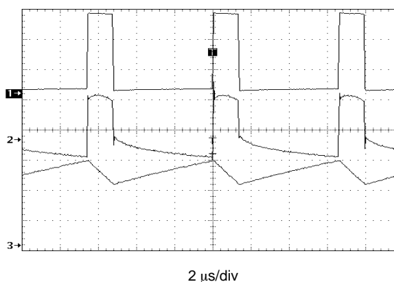
V_{OUT} = 5.0 \text{ V} , V_{in} = 1.5 \text{ V} , I_O = 60 \text{ mA} , L = 47 \text{ } \mu\text{H} , C_{OUT} = 68 \text{ } \mu\text{F} 1. V_{LX} , 2.0 V/div 2. V_{OUT} , 20 mV/div, AC coupled 3. I_L , 100 mA/div
