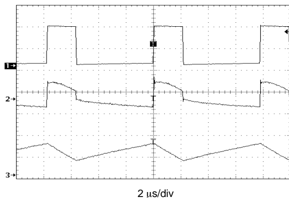
V_{OUT} = 3.0 \text{ V} , V_{in} = 1.2 \text{ V} , I_O = 30 \text{ mA} , L = 47 \text{ } \mu\text{H} , C_{OUT} = 68 \text{ } \mu\text{F} 1. V_{LX} , 2.0 V/div 2. V_{OUT} , 20 mV/div, AC coupled 3. I_L , 100 mA/div
