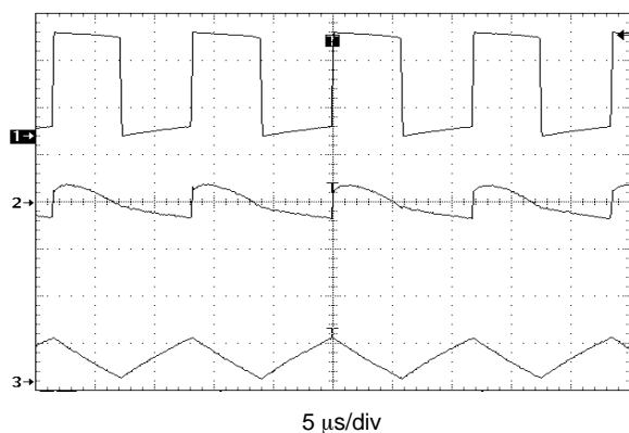
V_{OUT} = 1.9 \text{ V} , V_{in} = 1.2 \text{ V} , I_O = 30 \text{ mA} , L = 47 \text{ } \mu\text{H} , C_{OUT} = 68 \text{ } \mu\text{F} 1. V_{LX} , 1.0 V/div 2. V_{OUT} , 20 mV/div, AC coupled 3. I_L , 100 mA/div
