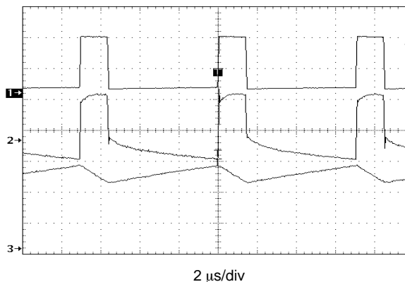
V_{OUT} = 3.0 \text{ V} , V_{in} = 1.2 \text{ V} , I_O = 70 \text{ mA} , L = 47 \text{ } \mu\text{H} , C_{OUT} = 68 \text{ } \mu\text{F} 1. V_{LX} , 2.0 V/div 2. V_{OUT} , 20 mV/div, AC coupled 3. I_L , 100 mA/div
