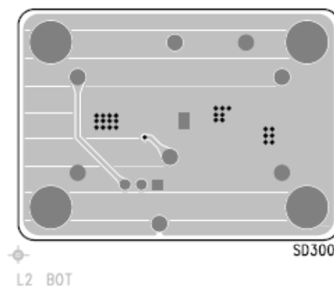
Figure 3. Bottom Layer
