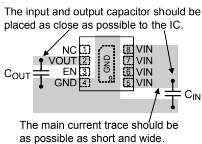
Figure 4. PCB Layout for WDFN Package
