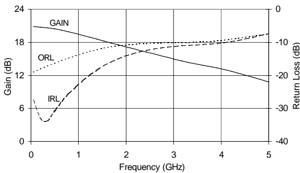
Gain & Return Loss vs. Frequency V_D = 5.1 \text{ V} , I_D = 75 \text{ mA} (Typ.)
