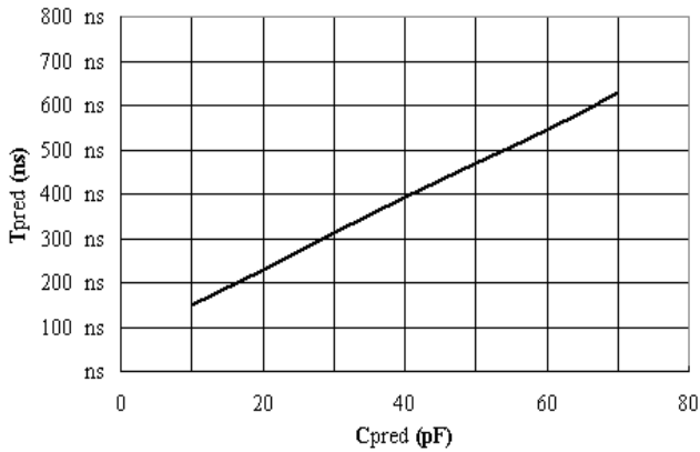
Figure 3 : T_{pred} vs C_{pred} @ Freq =100 KHz ; V_{DD} =10V
