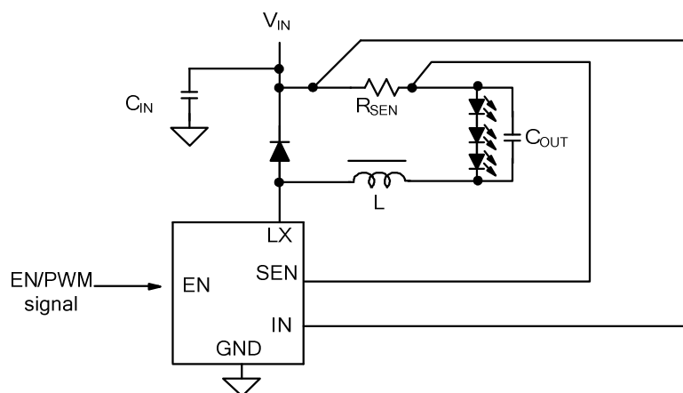
Figure 1. Schematic diagram
