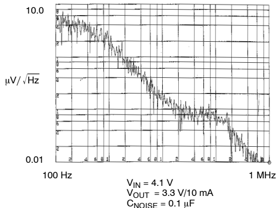
Noise Spectrum
