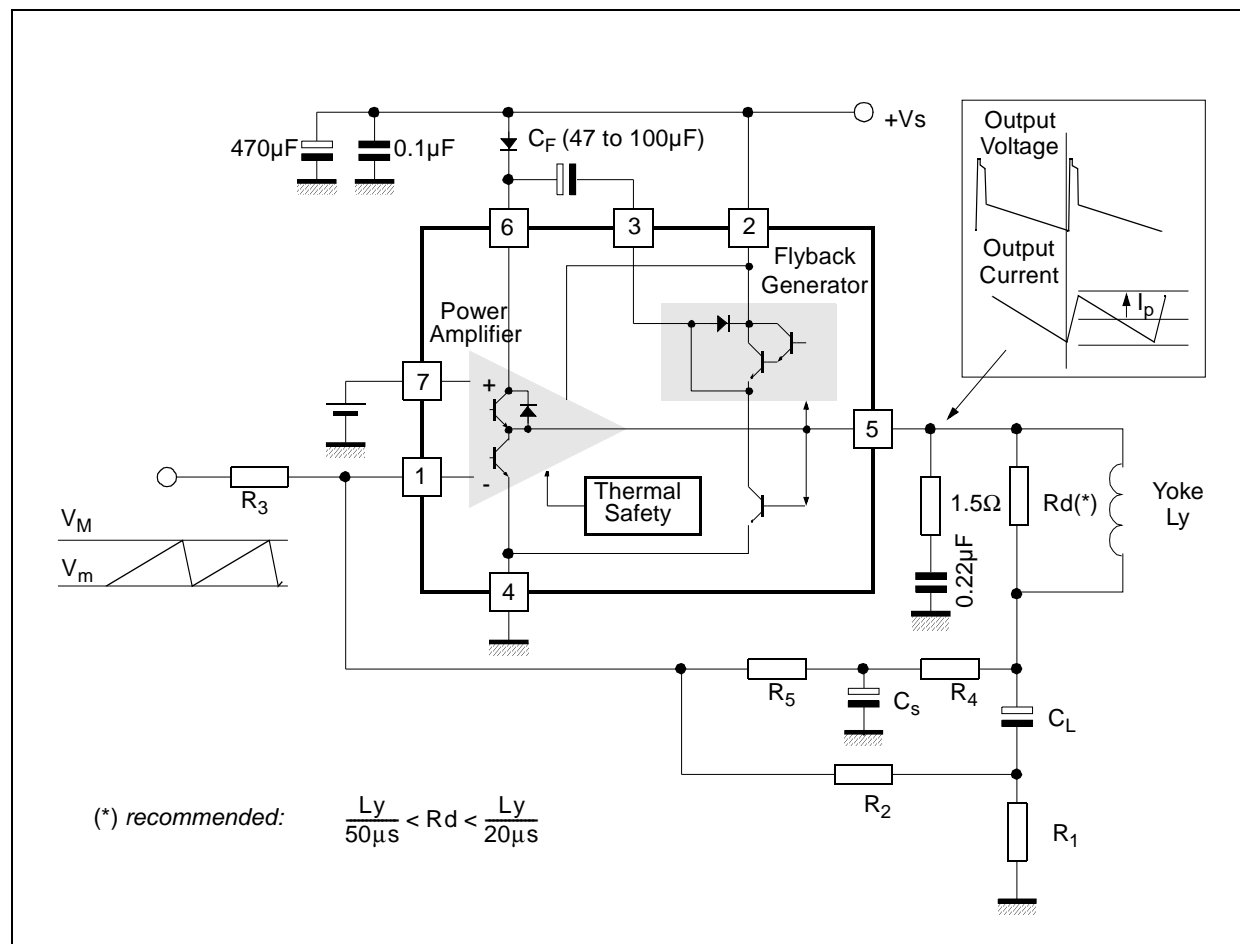
Figure 6: AC-coupled Application
