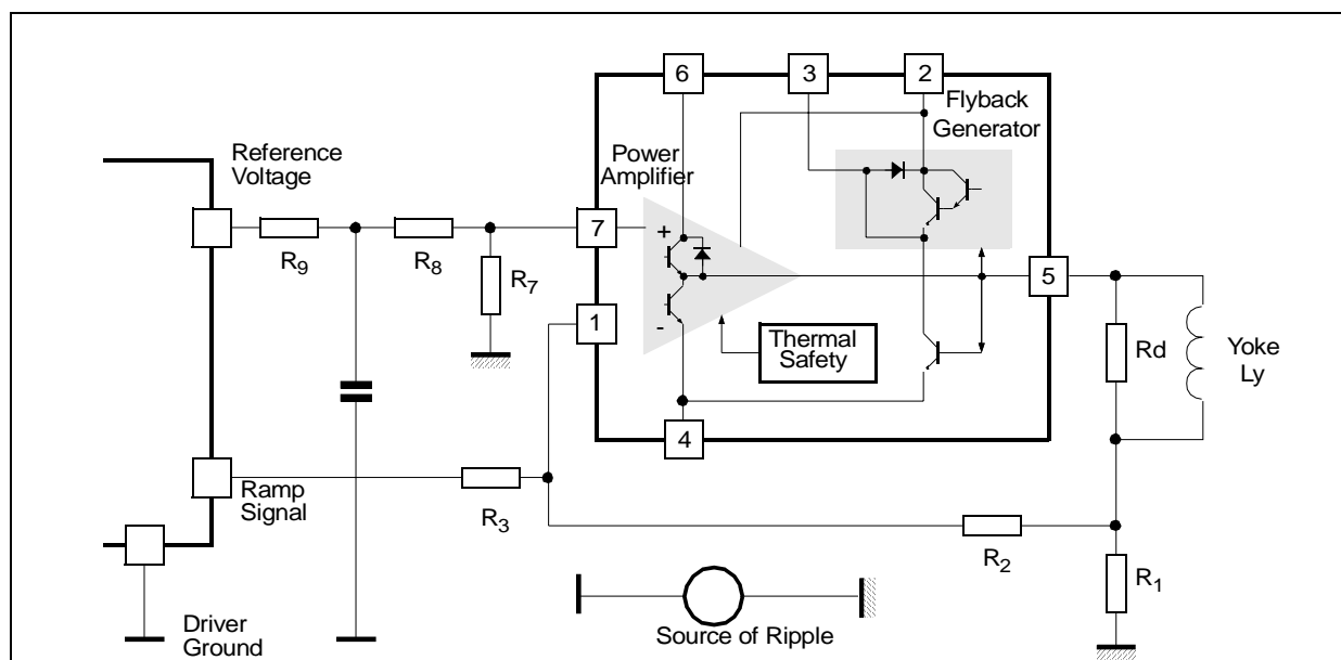
Figure 5: Ripple Rejection
