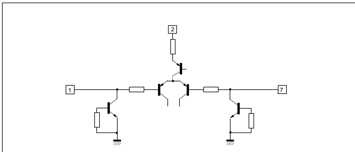
Figure 11: Pins 1 and 7
