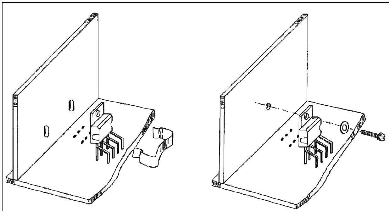
Figure 10: Mounting Examples
