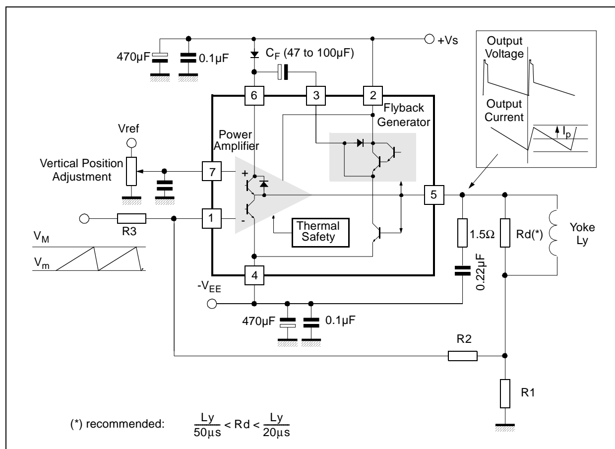
Figure 4: DC-coupled Application
