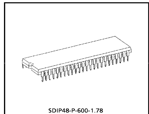
SDIP48-P-600-1.78
