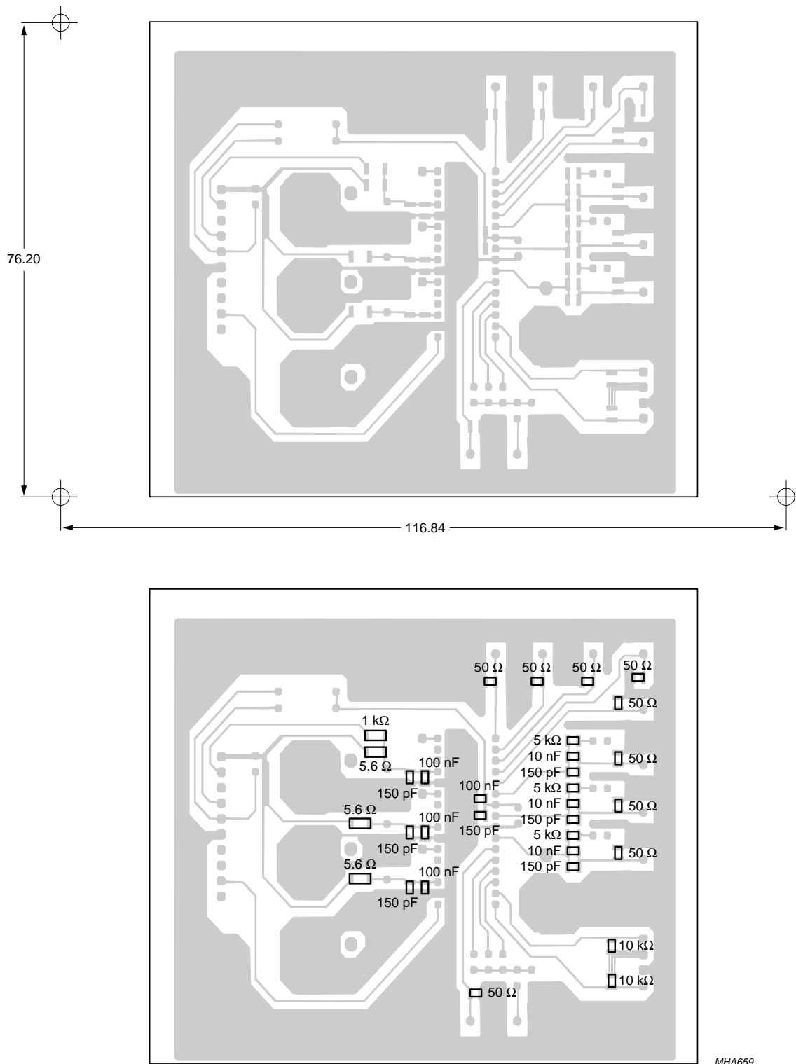
Fig.21 Component layout and printed-circuit board; side B (for side A see Fig.20).
