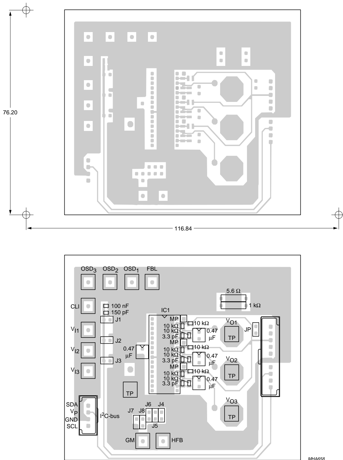
Fig.20 Component layout and printed-circuit board; side A (for side B see Fig.21).
