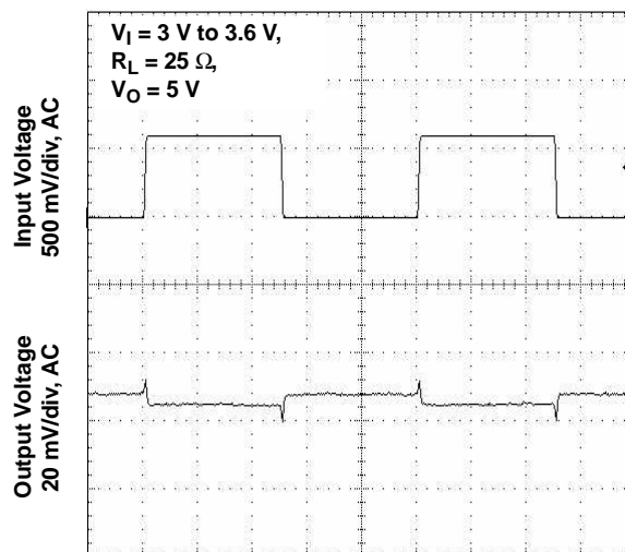
TPS61027 LINE TRANSIENT RESPONSE
