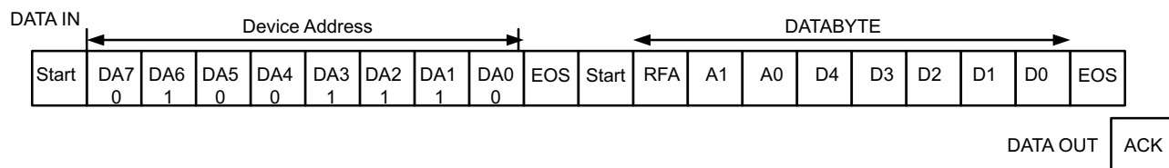
Figure 34. EasyScale™ Protocol Overview
