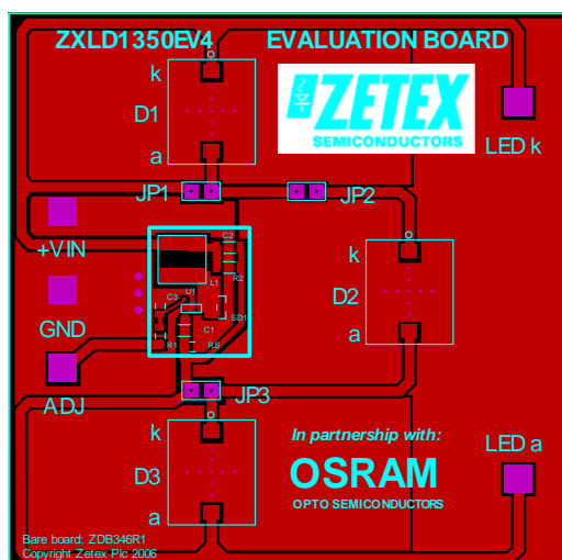
Figure 3: Top View
