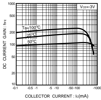
Fig.7 DC current gain vs. collector current
