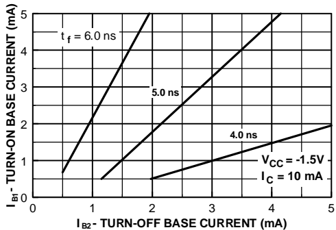
Fall Time vs. Turn-On / Turn-Off Base Currents
