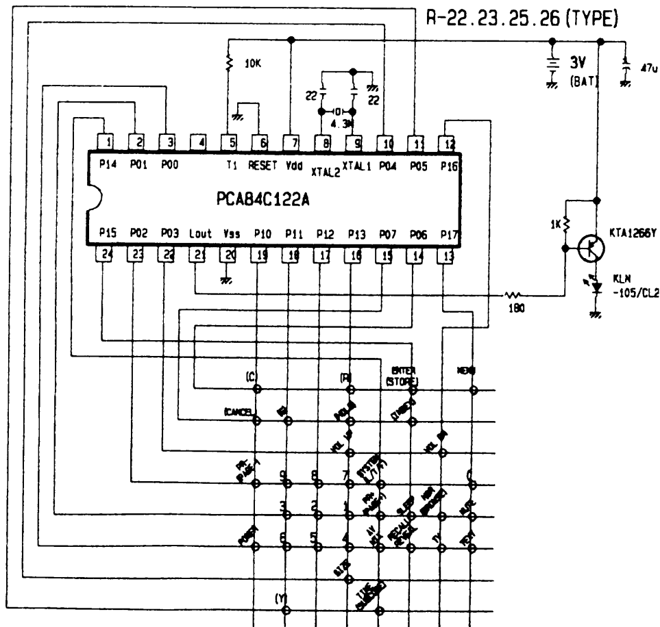
Remote Control Diagram
